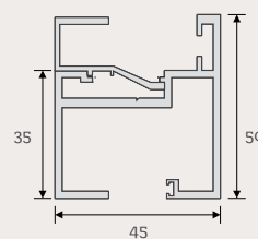
Door Rebate Profile with over panel clip
